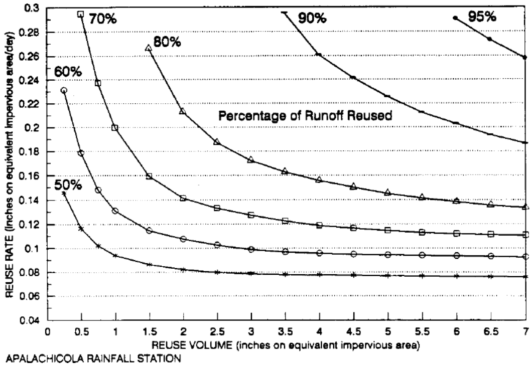
Figure 4-1 Rate-Efficiency-Volume (REV) Curves for Apalachicola.
