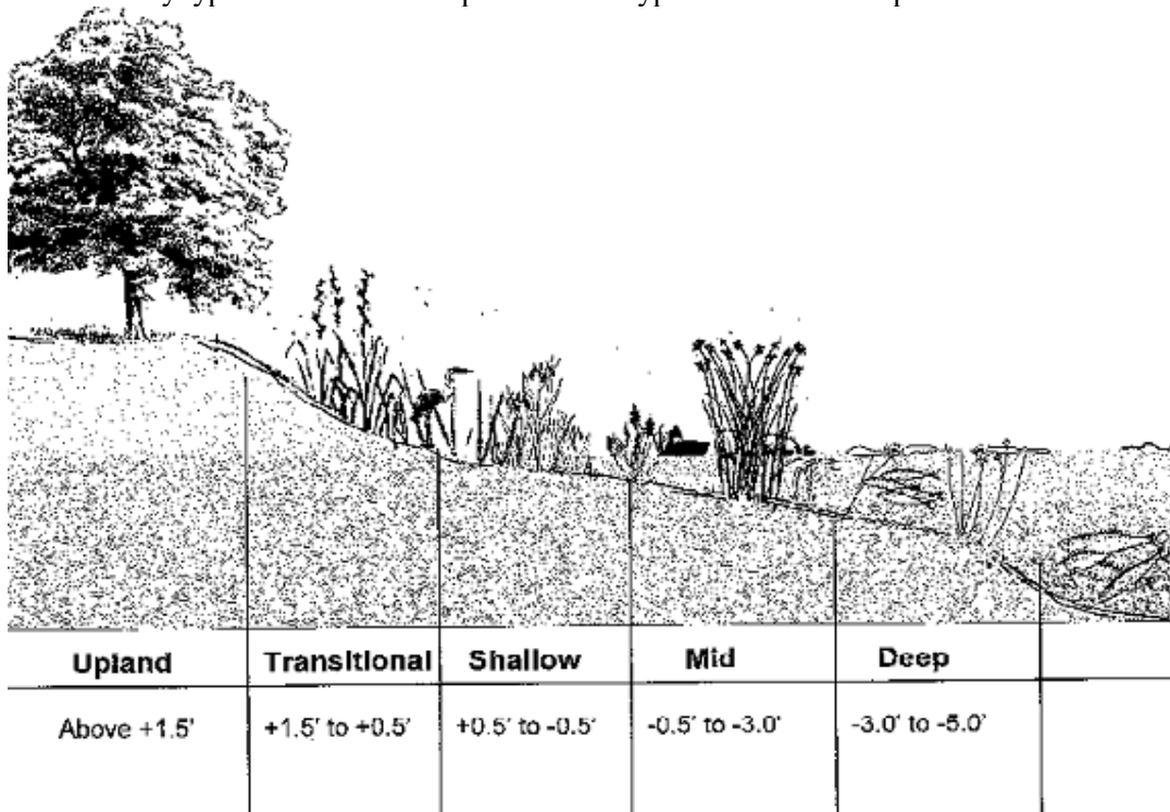
Figure 3-2 Community Types or Zones for Littoral Shelf Plantings
