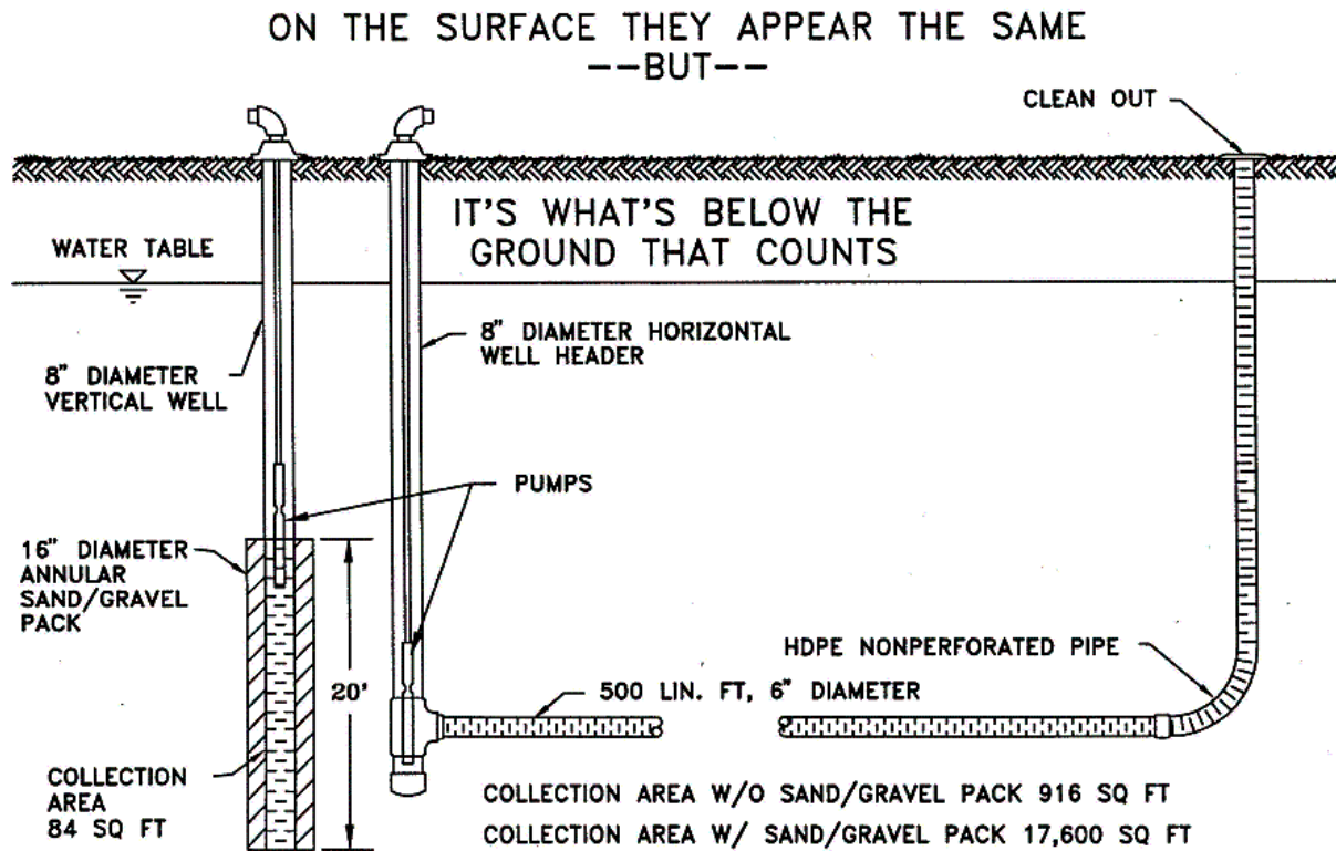
Figure 4-1. Schematic for Harvesting Water Withdrawal System.
