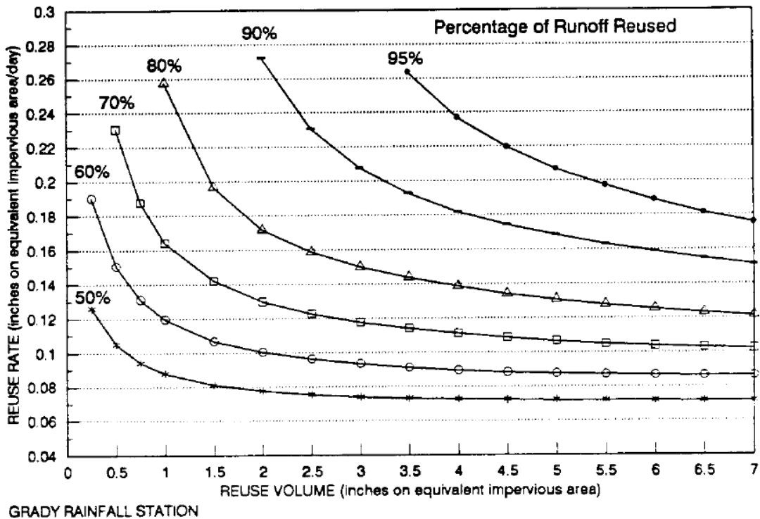
Figure 4-2 Rate-Efficiency-Volume (REV) Curves for Grady.
