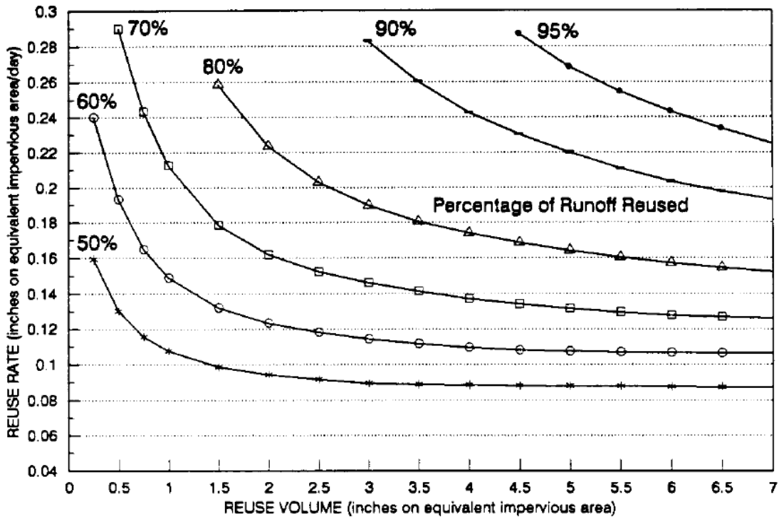
Figure 4-3 Rate-Efficiency-Volume (REV) Curves for Niceville.
